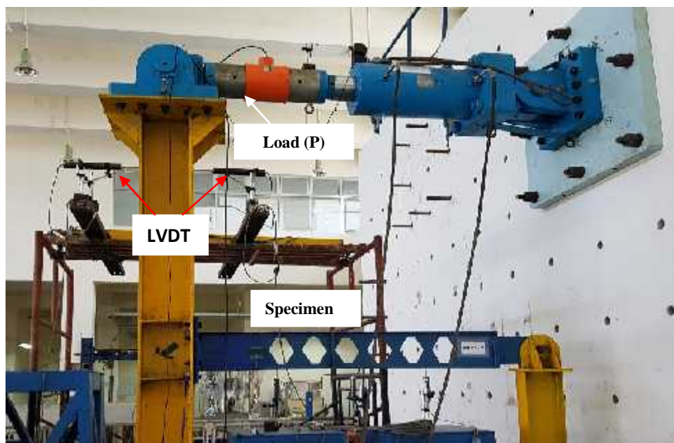
Figure 5. The instrument of the castellated beam-column testing.
