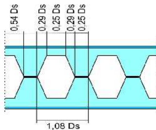
Figure 1. Standard of the castellated beam.
