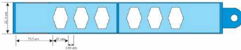
Figure 2. Location of castellated beam opening distance.
